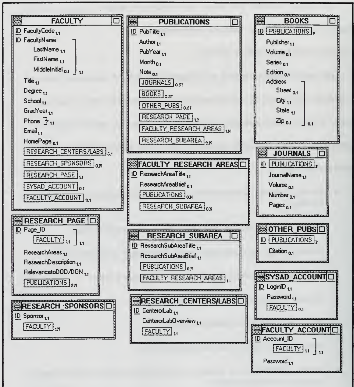
Figure 2. Semantic Object Model
